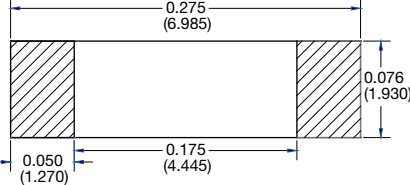
2208 Land Pattern
