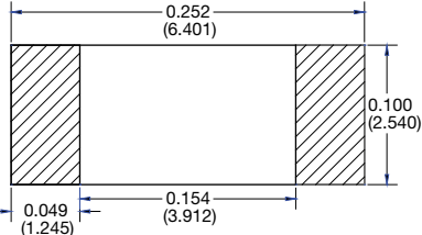
2010 Land Pattern
